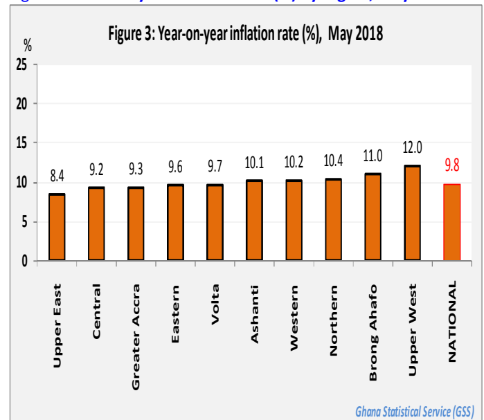
Figure 3: Year-on-year Inflation rate (%) by region, May 2018
