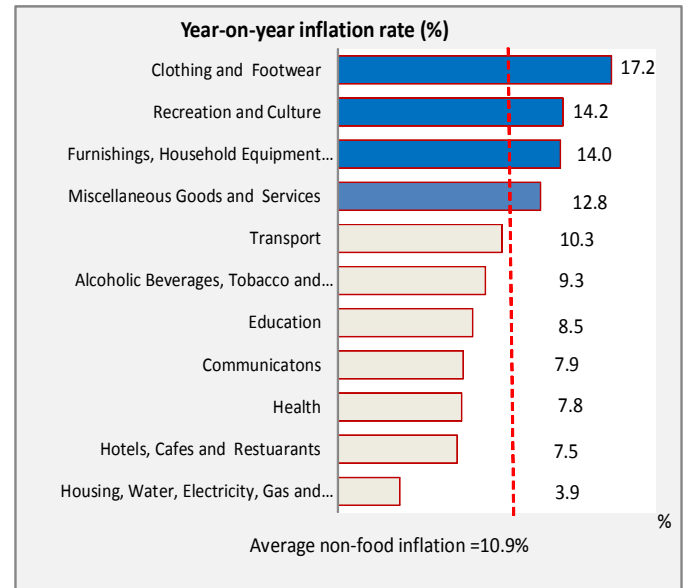
Figure 2: Year-on-year Non-Food Inflation (%) by major subgroups, May 2018
