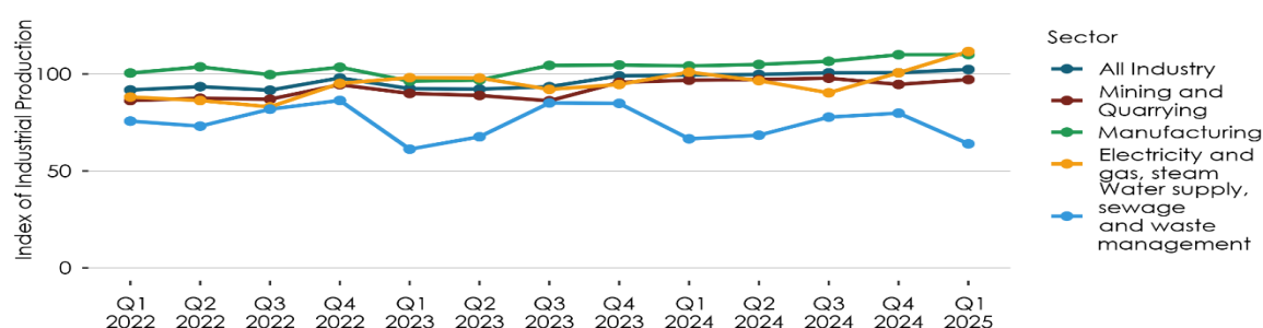
Figure 1: Trend in IIP by Sub-Sector
