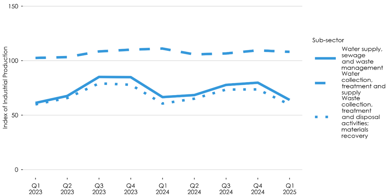
Figure 4: Trend in IIP for Water Supply, Sewerage and Waste Management Sub-sector
