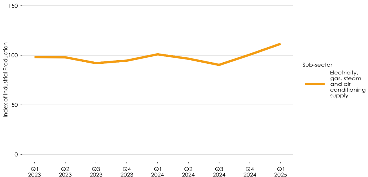
Figure 3: Trend in IIP for Electricity and Gas Sub-sector
